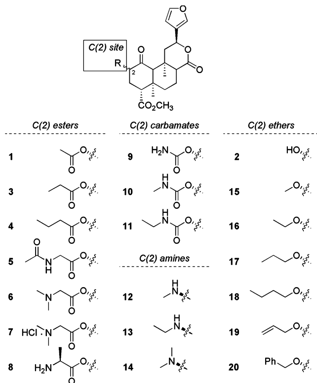
Figure 1. Salvinorin derivatives selected for study.
