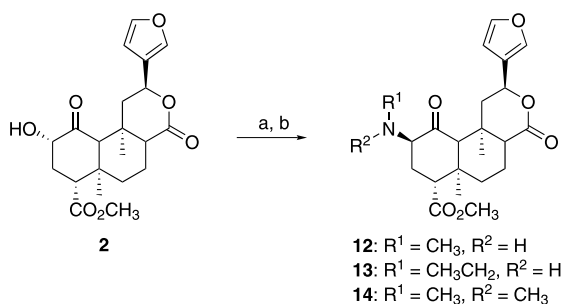
Scheme 3. Syntheses of C(2) amines. Reagents and conditions: (a) (\text{CF}_3\text{SO}_2)_2\text{O} , pyridine, \text{CH}_2\text{Cl}_2 ; (b) \text{R}^1\text{R}^2\text{NH} , THF, 26–29%, over two steps.
