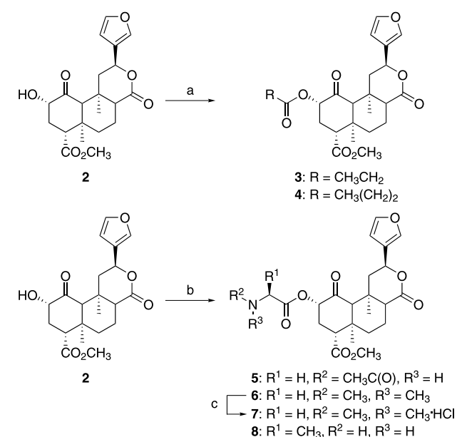
Scheme 1. Syntheses of C(2) esters. Reagents and conditions: (a) appropriate acyl chlorides, pyridine, 36–61%; (b) appropriate amino acids, DCC or EDCI, DMAP, \text{CH}_2\text{Cl}_2 (followed by deprotection with piperidine for the preparation of 8 ), 51–91%; (c) HCl, \text{Et}_2\text{O} , 58%.
