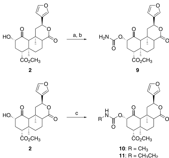
Scheme 2. Syntheses of C(2) carbamates. Reagents and conditions: (a) \text{CCl}_3\text{C(O)NCO} , \text{CH}_2\text{Cl}_2 ; (b) \text{Al}_2\text{O}_3 , 91%, over two steps; (c) appropriate isocyanates, DMAP, pyridine, 53–68%.
