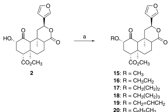
Scheme 4. Syntheses of C(2) ethers. Reagents and conditions: (a) appropriate alkyl iodide (or bromide for 20 ), \text{Ag}_2\text{O} , \text{CH}_3\text{CN} , 36–77%.
